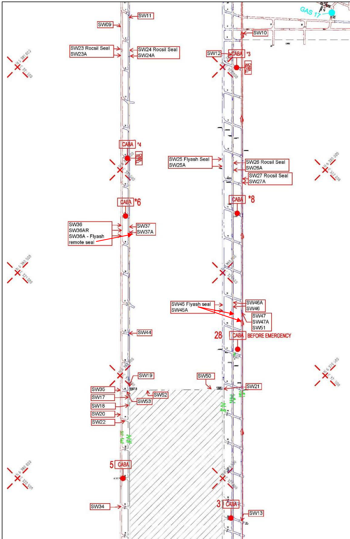
Figure 9: Boreholes used to seal LW1 and monitor the conditions underground
