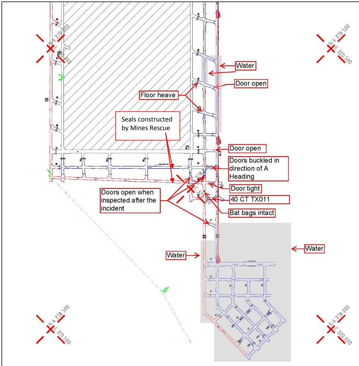
Figure 20: Mine plan showing conditions upon re-entry in the maingate behind the longwall
