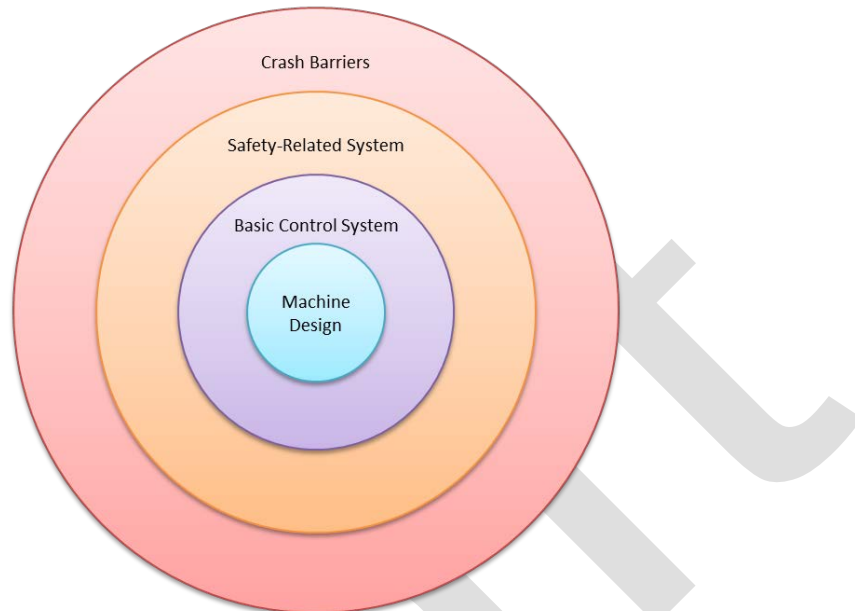
Figure 5: An example of a “layers of protection” diagram applied to a winding system.
